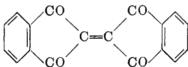
VIII Bis-1,3-diketoindoxylidene
