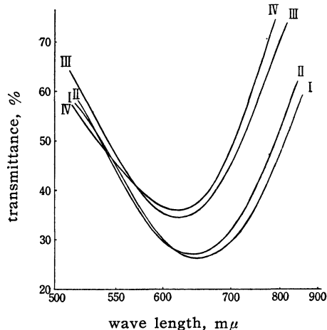
Fig. 2. Absorption spectra of various copper salts (10 \mu M/ml. of 8% \text{Na}_2\text{CO}_3 solution). (I), copper glycinate; (II), (I) + \text{CH}_3\text{CHO} at the beginning of the reaction; (III), (I) + \text{CH}_3\text{CHO} after the reaction; (IV) copper threoninate.
